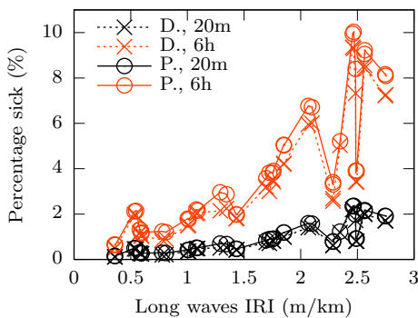
Figure 11. Relationship between the probability that untrained occupants will be sick from nausea and the Long Waves IRI for all profiles.
